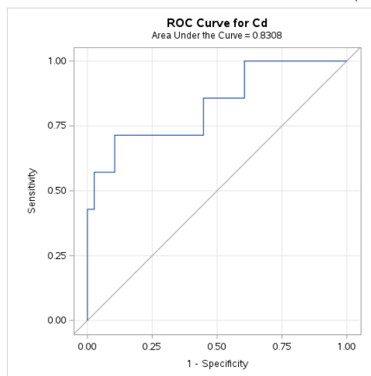
Figure 3: Receiver Operating Characteristic (ROC) Curve for classifying smokers based on the Cadmium concentrations in blood donors (n=45)
